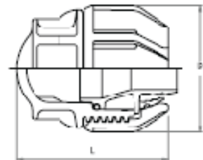
3/4" END CAP
